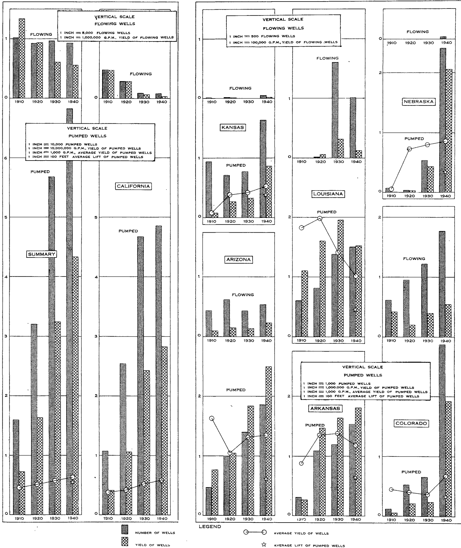
CHART XIII. — NUMBER AND YIELD OF PUMPED AND FLOWING WELLS, AVERAGE YIELD OF PUMPED WELLS, 1910 TO 1940; AND AVERAGE LIFT OF PUMPED WELLS, 1940: BY STATES
