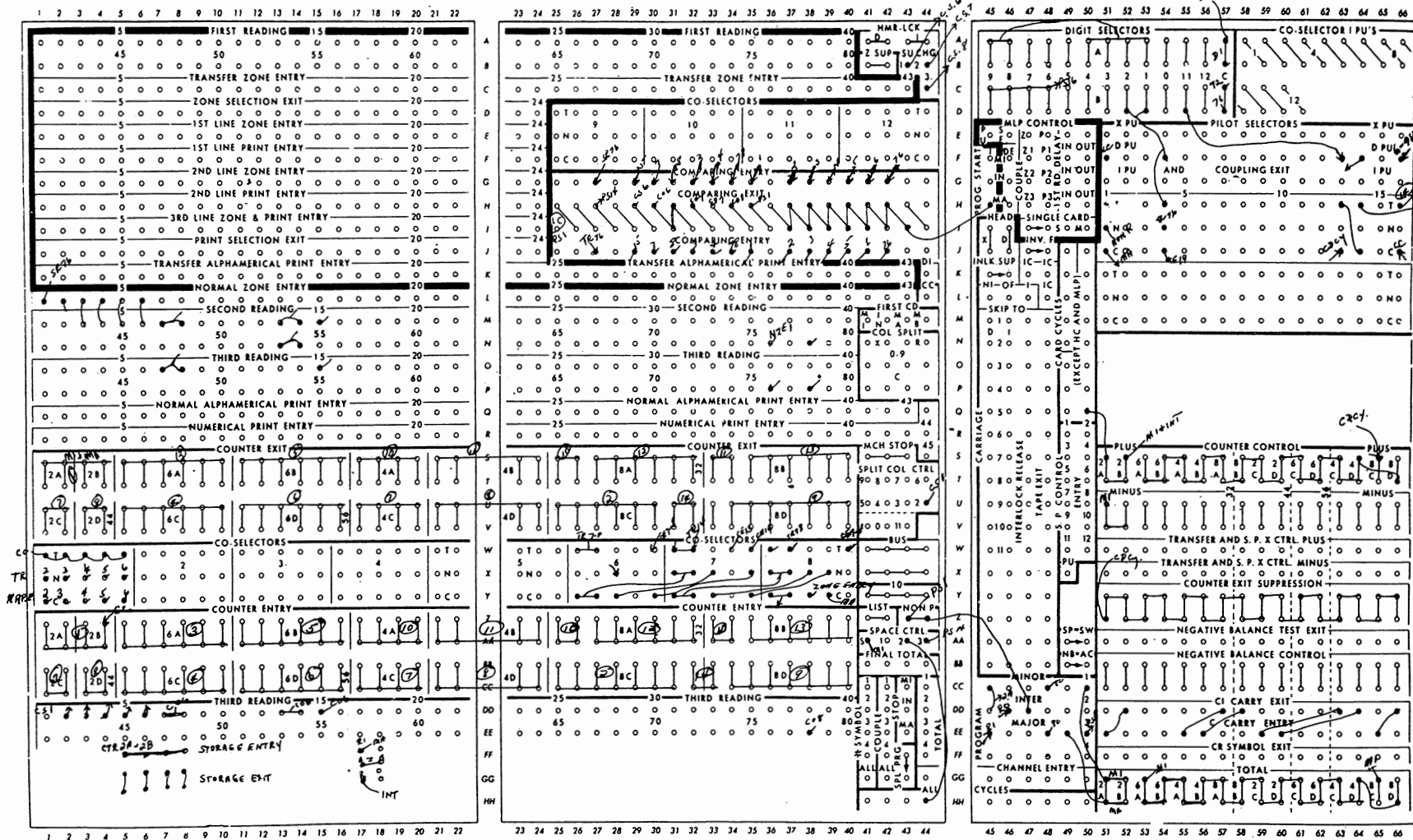
FIGURE 45.—Illustrative example of wiring diagram, type 402-403, control panel.
