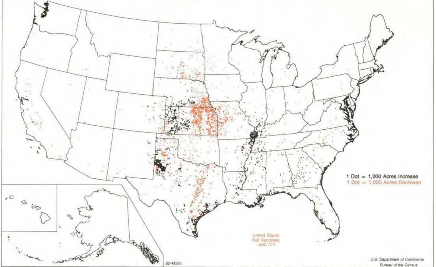
Sorghum Harvested for All Purposes - Change in Acreage: 1978 to 1982
