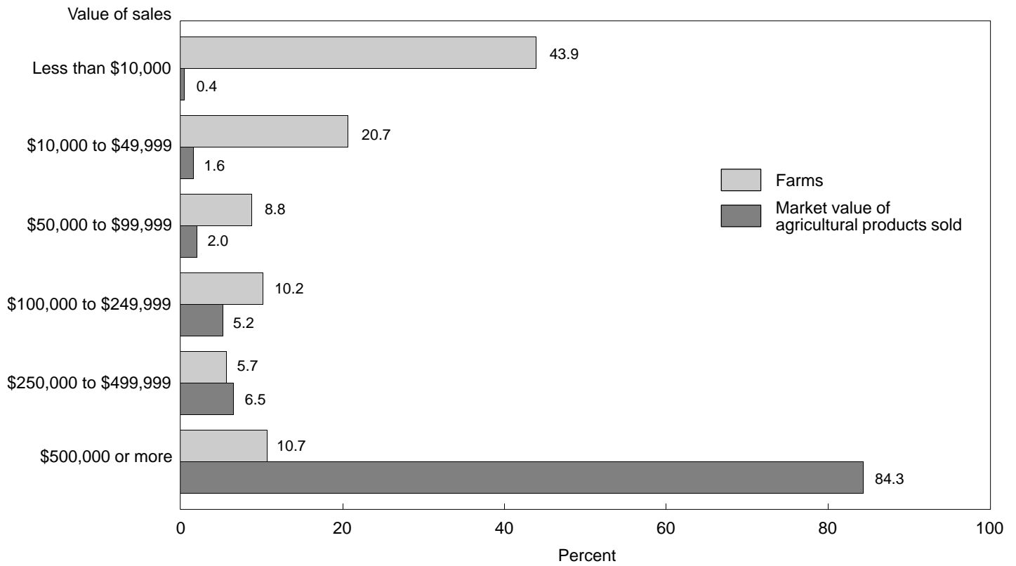
Figure 3. Farms by Market Value of Agricultural Products Sold: 1969 to 1997
