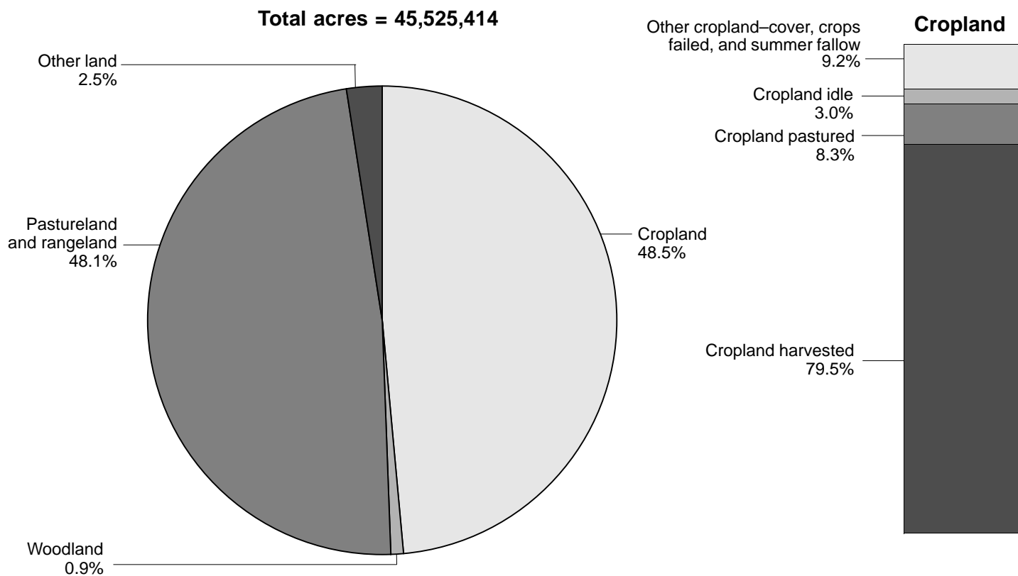
Figure 4. Land Use: 1997
