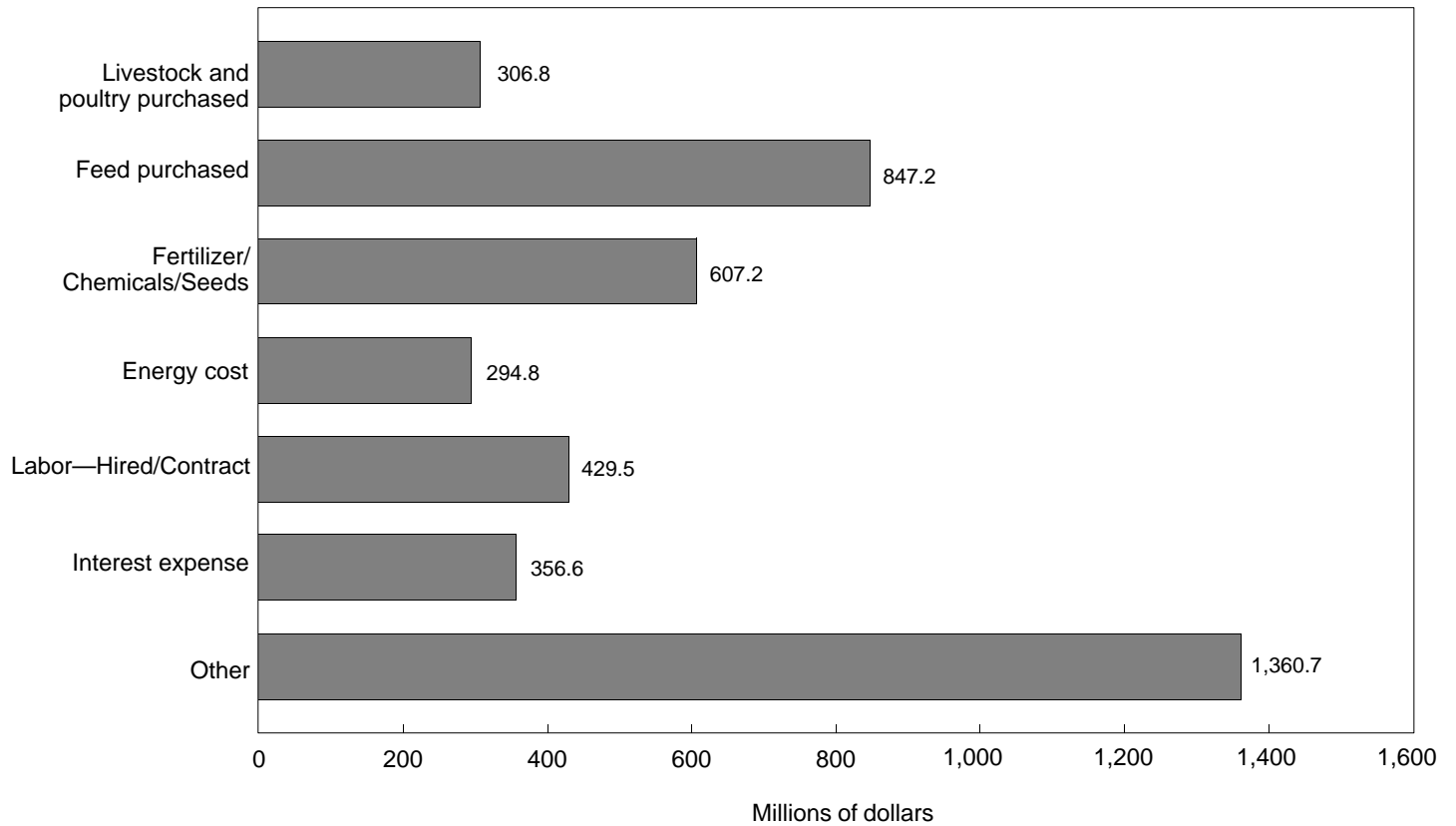
Figure 7. Production Expenses: 1997
